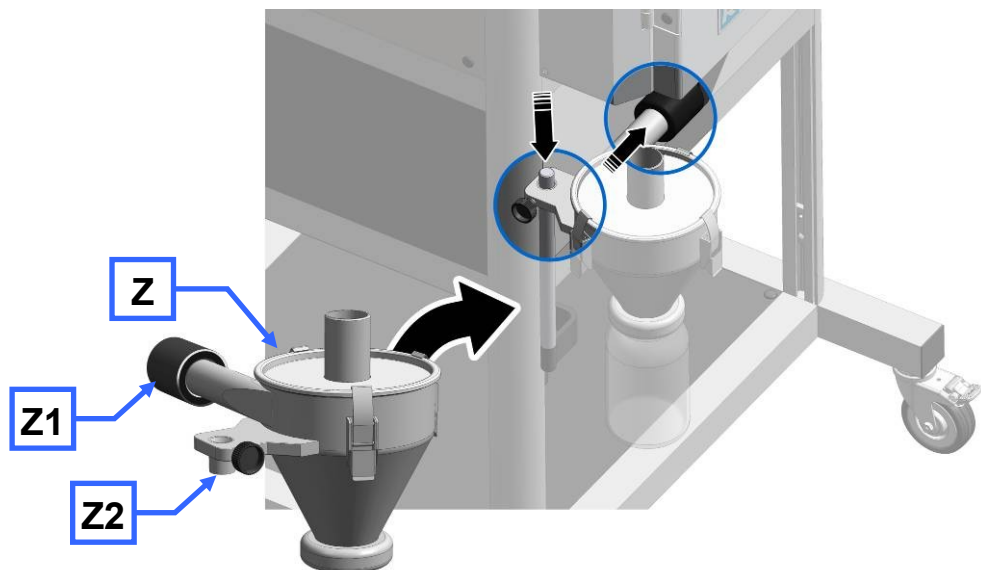
Figure 7 : Installation du cyclone
