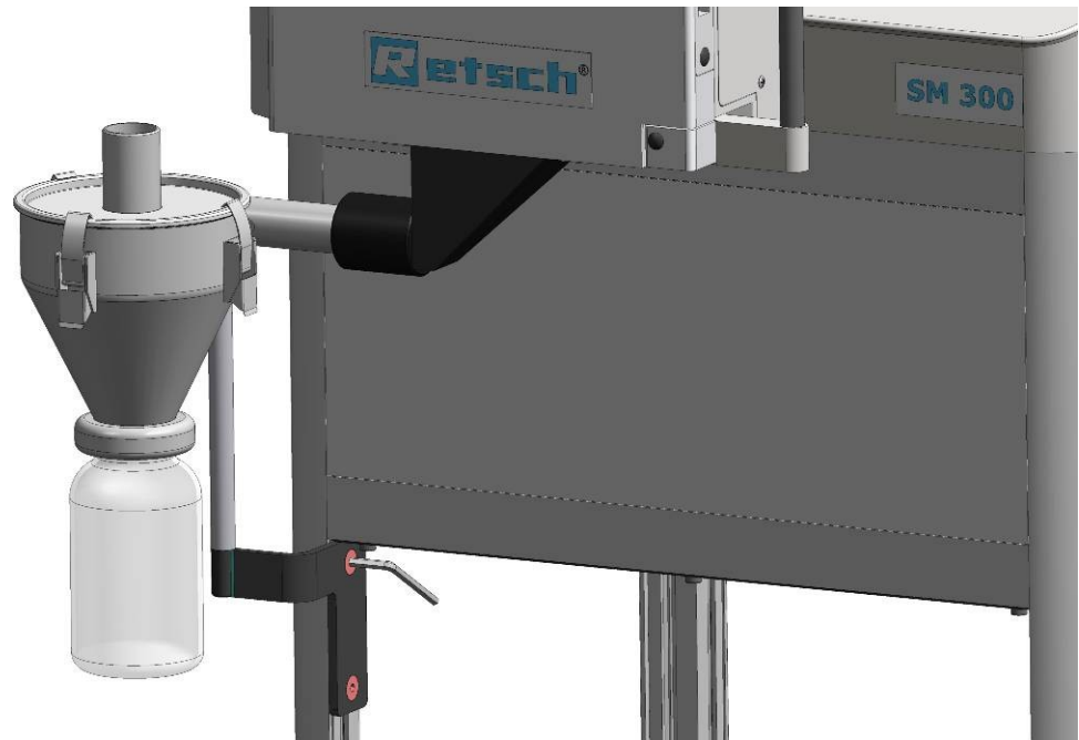
Figure 8 : Cyclone monté
